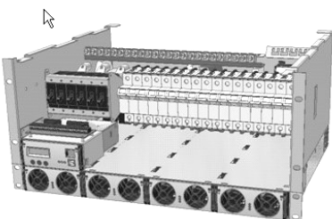
Flatpack2 5U Integrated System
