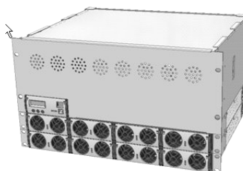
Flatpack2 6U Integrated System
